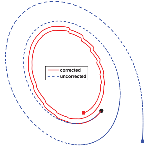
FIG. 4. (Color online) The first 20 min of a forecast for an initial state attracted to the left-lobe convective equilibrium stabilized by the empirical correction (i.e., one of the dark red dots near the center of the left lobe in the bottom of Fig. 3). The uncorrected EM model trajectory (blue dash) behaves as it should, winding away from the equilibrium at the center of the lobe, whereas the trajectory of the corrected model (solid red) collapses toward the equilibrium solution, indicating false stability produced by correction. The source of the false stability is the overcorrective nudging visible as jumps (every 30 s, the length of the analysis window) on the red curve. The correction is attempting to lengthen flow regimes, a consequence of the blue regions near the equilibria in the top of Fig. 3.
